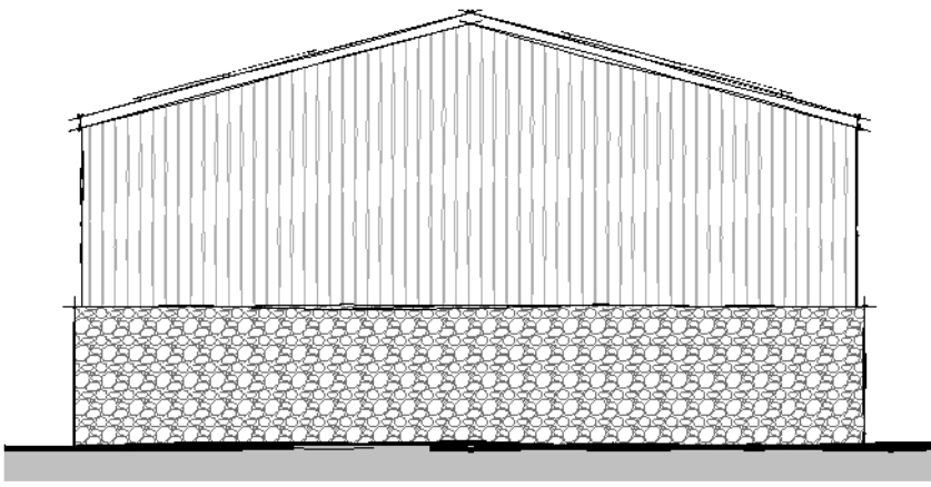
Side Elevation 02 1 : 100
