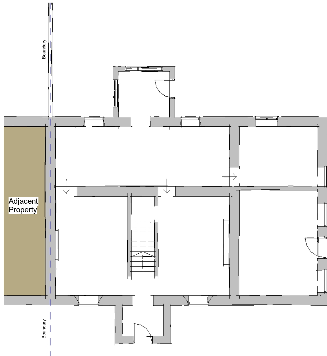
Ground 1 : 100
