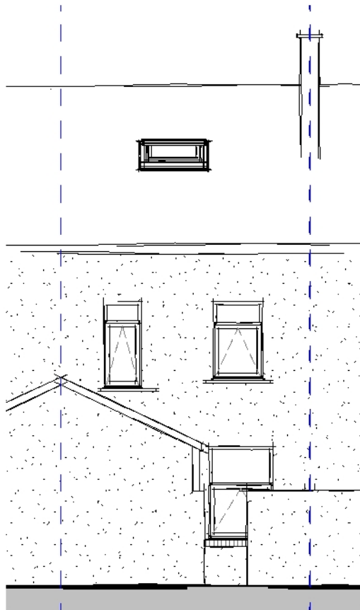
Rear Elevation 1 : 100
