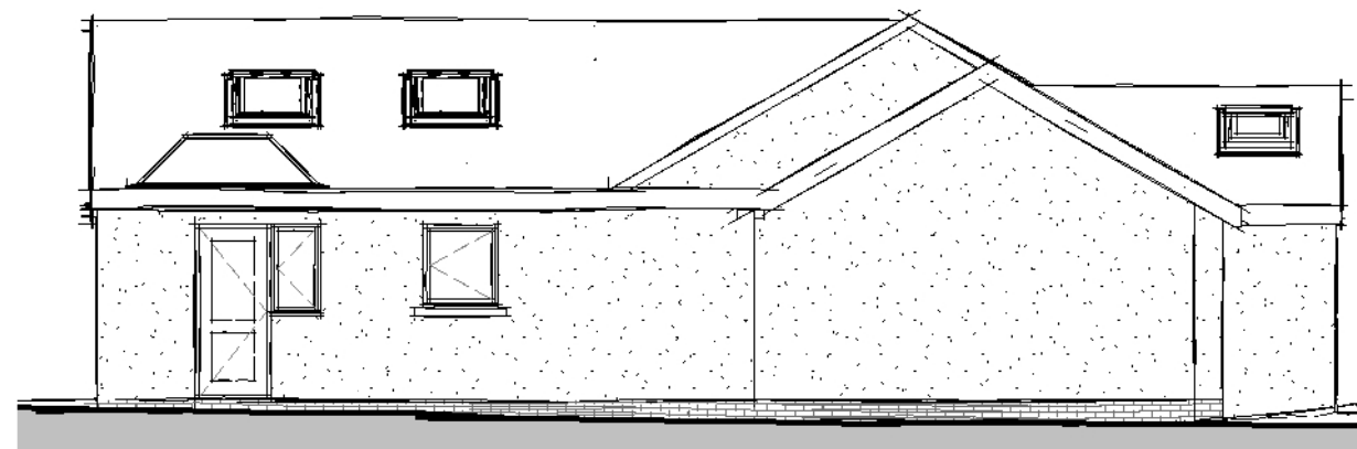
Side Elevation 02
