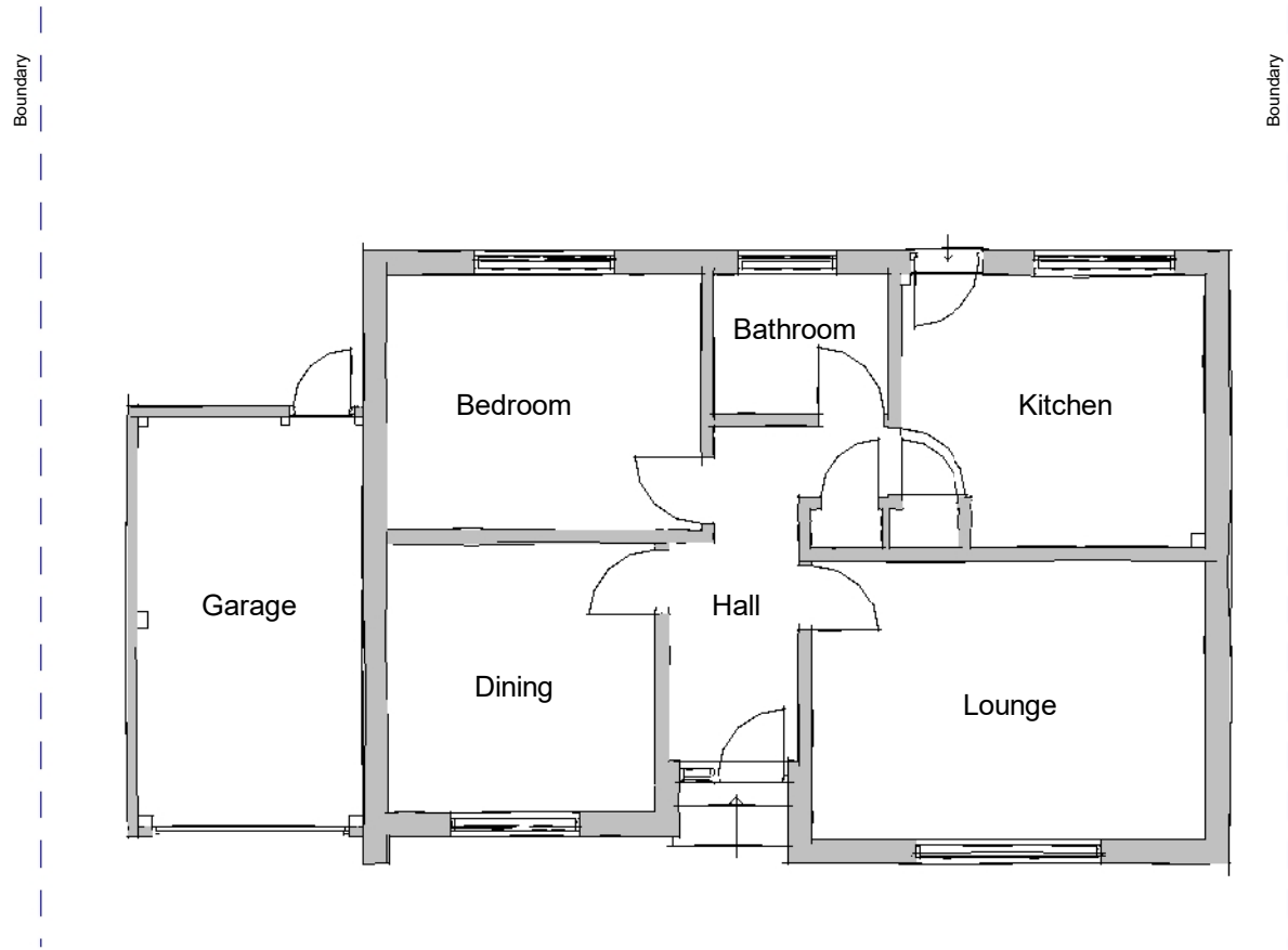
Ground 1 : 100
