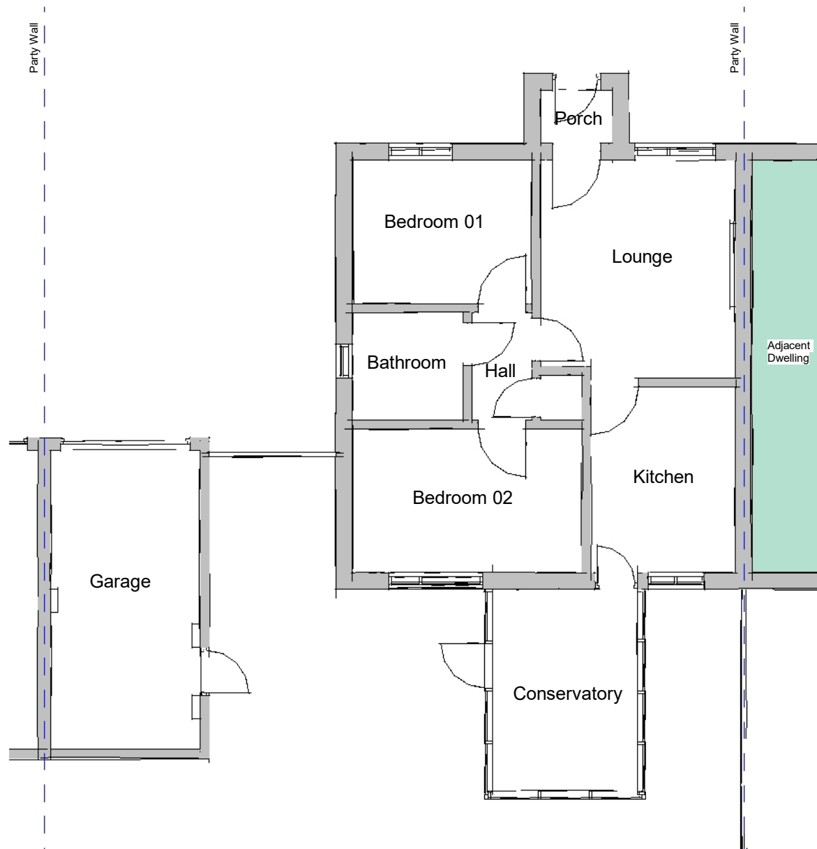
Ground 1 : 100
