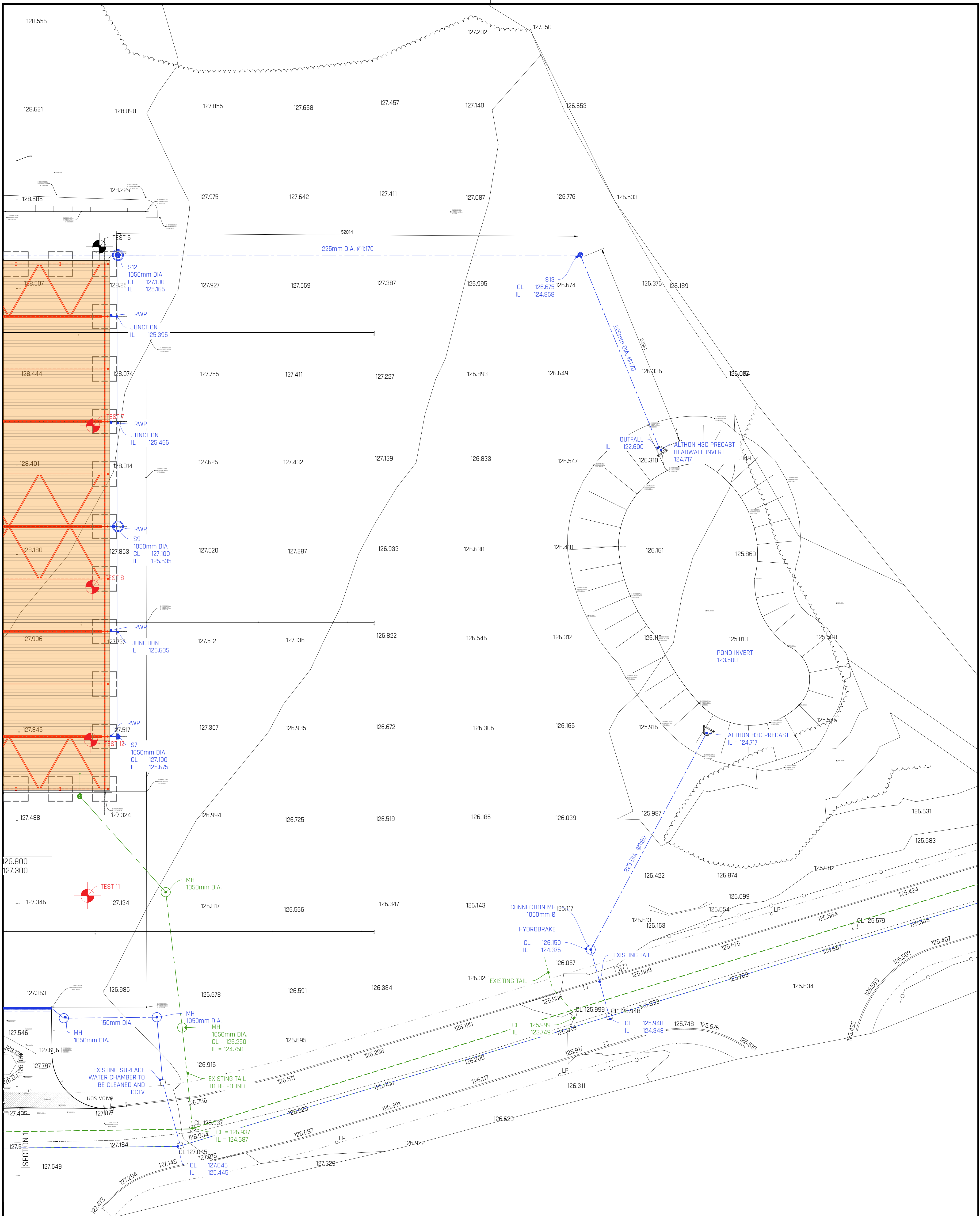
PLAN SCALE 1:200
