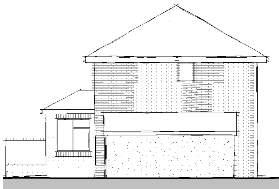
Side Elevation 02
