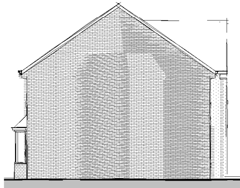
Side Elevation 02 1 : 100
