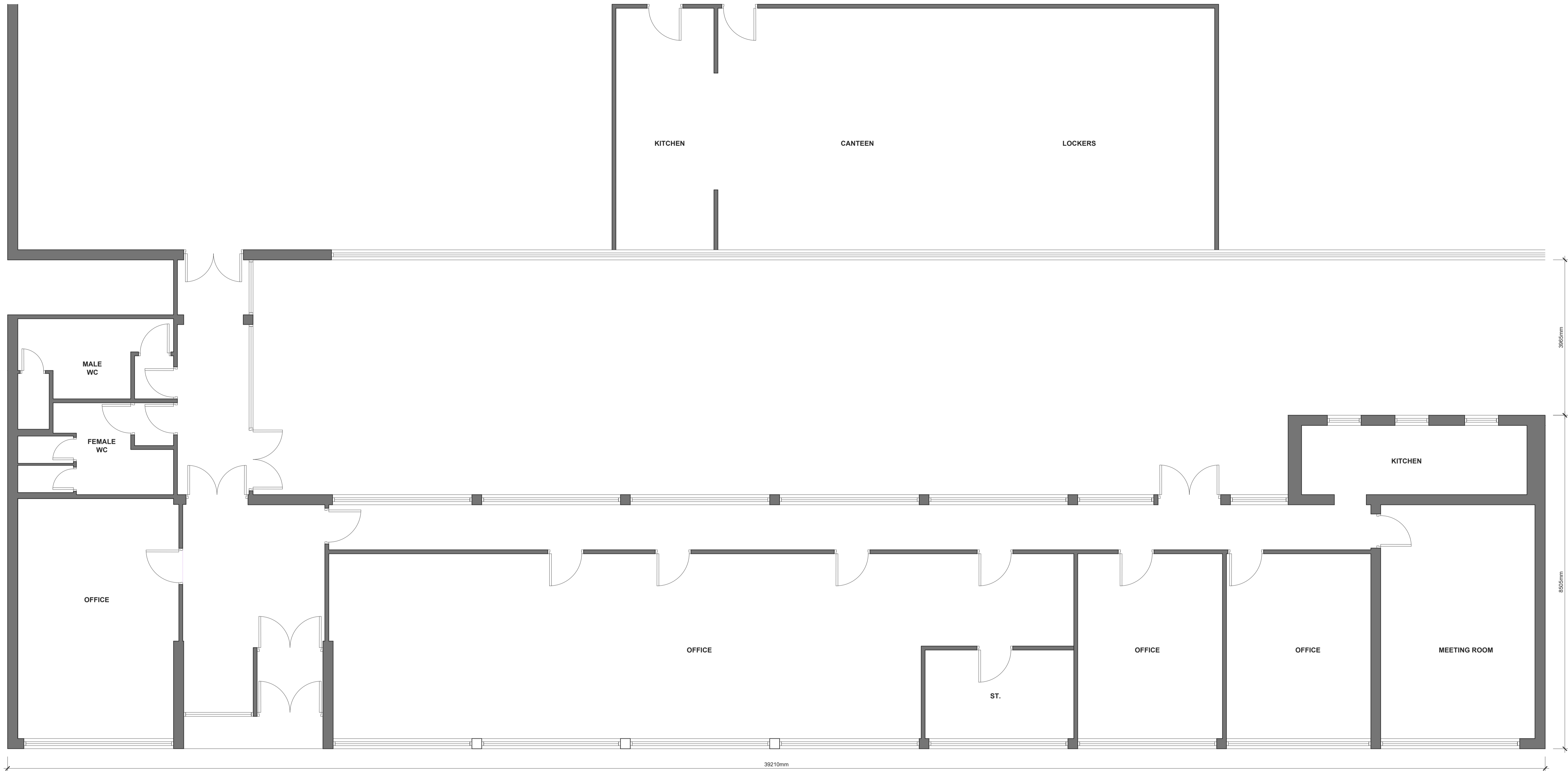
EXISTING PART GROUND FLOOR PLAN Scale 1:50
