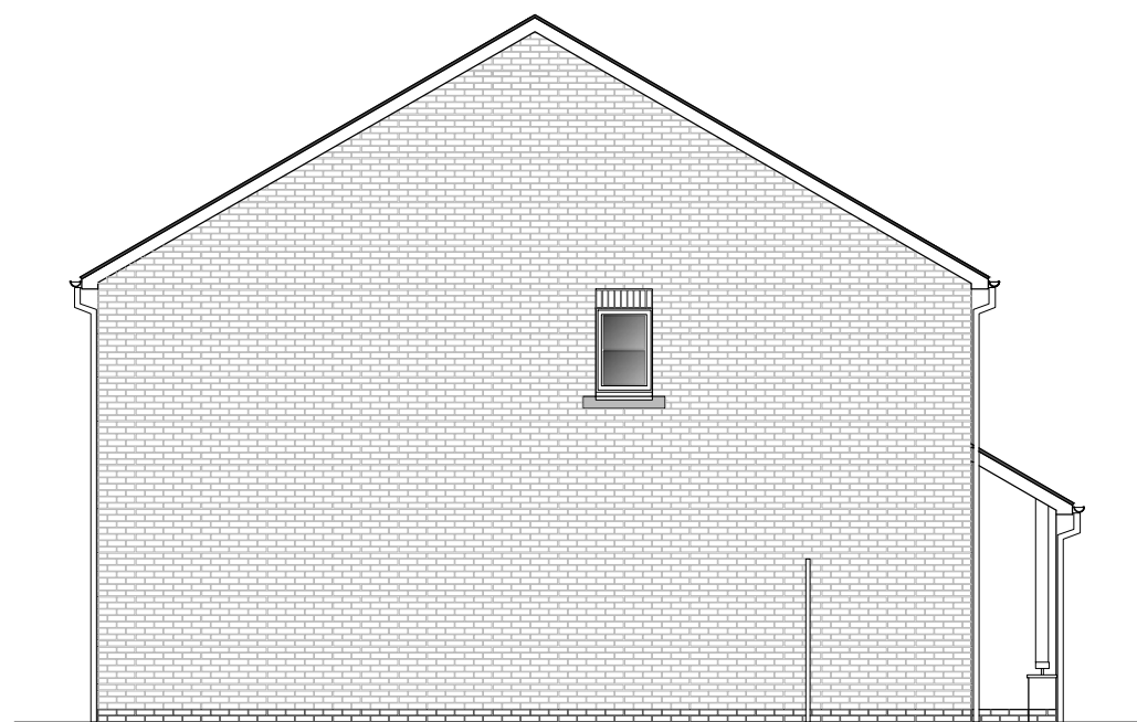
SIDE ELEVATION (LHS)
