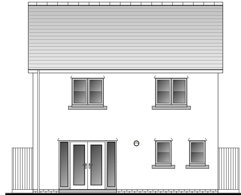
REAR ELEVATION
