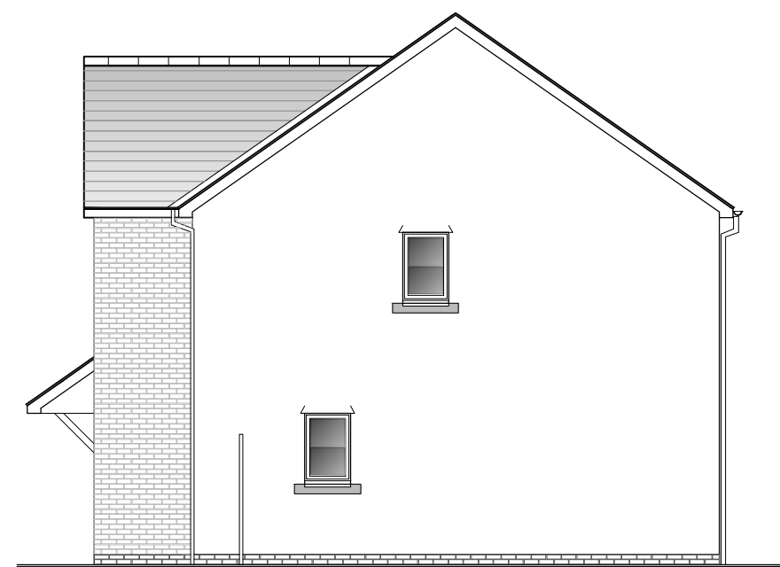
SIDE ELEVATION (RHS)
