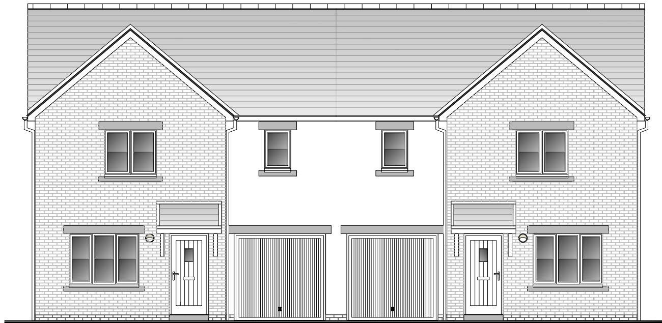
FRONT ELEVATION
