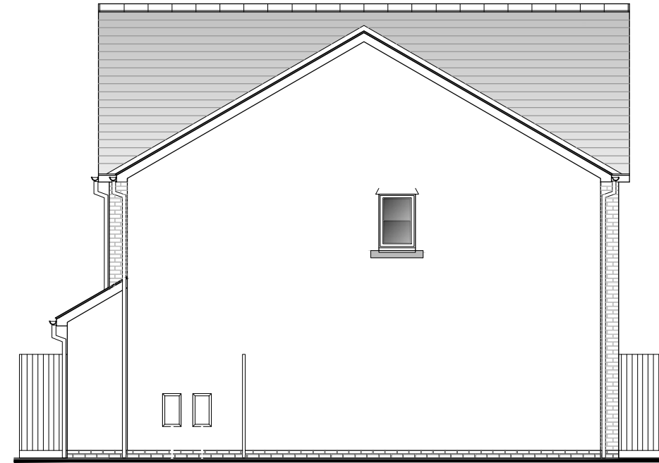
SIDE ELEVATION (RHS - ALDER)
