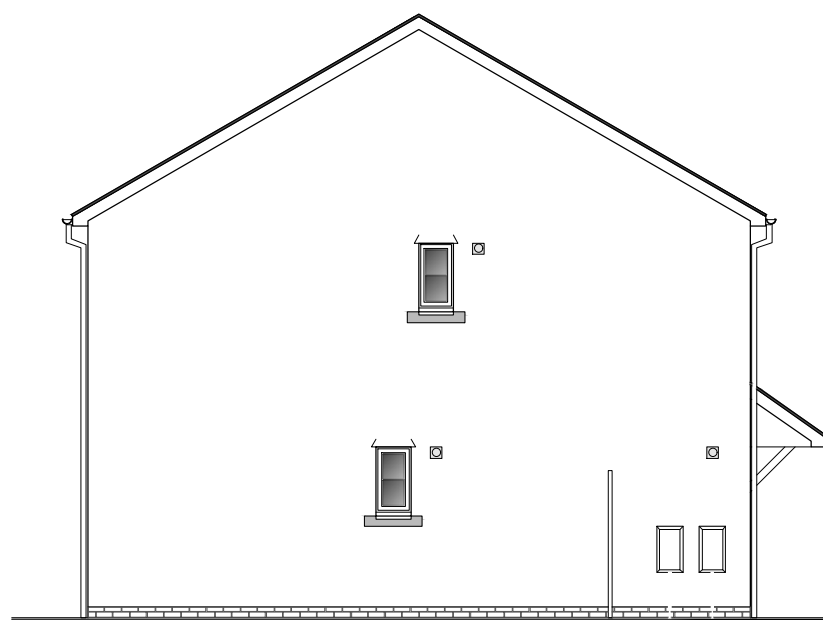
SIDE ELEVATION (LHS)
