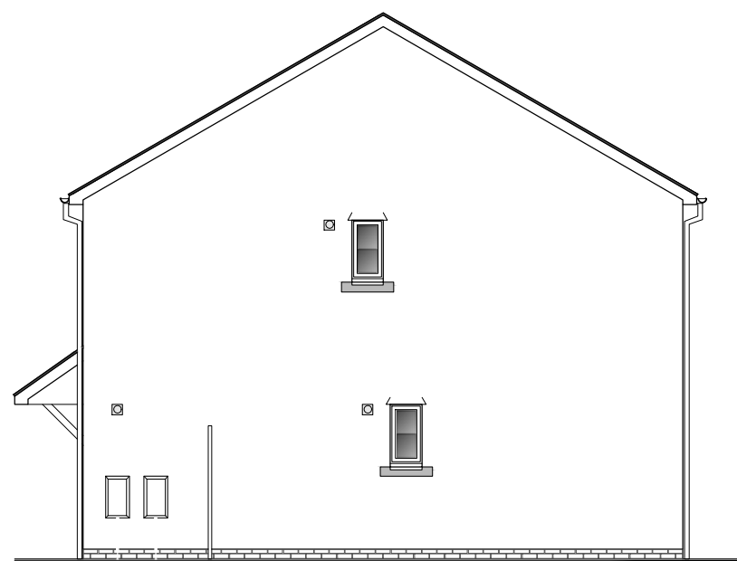
SIDE ELEVATION (RHS)
