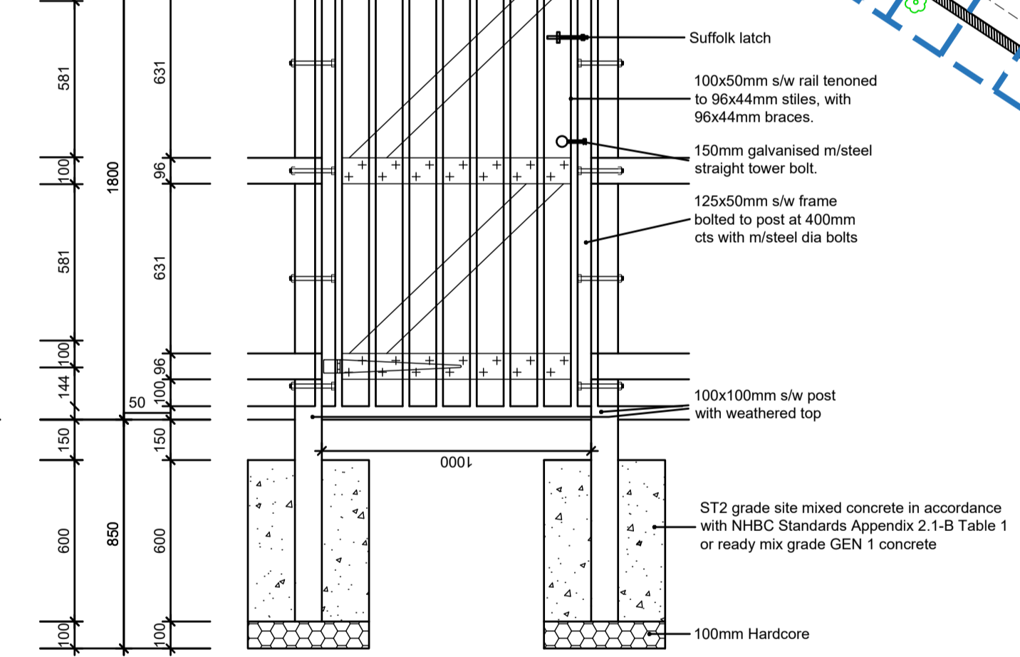
Type 1 - 1.8m High Fence Gate to Rear Gardens
