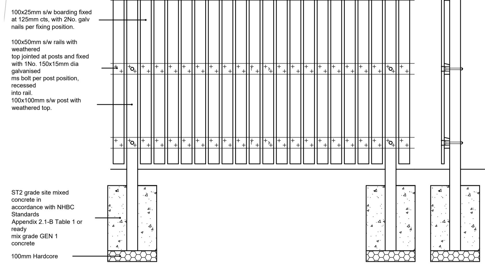
Type 1 - 1.8m Vertical Close Boarded Fence (Single Sided)
