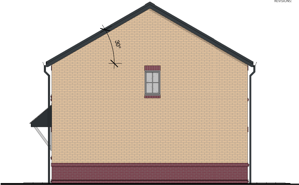
Side Elevation 1:100
