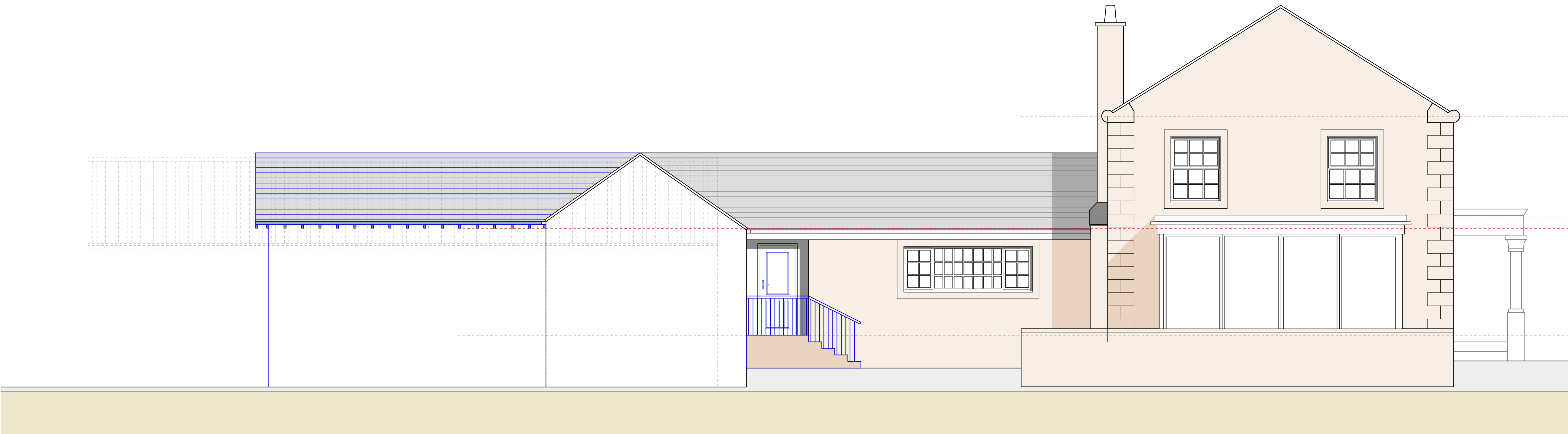
4 ELEVATION - PROPOSED SIDE B (NORTH FACING) SCALE 1:50 @ A1
