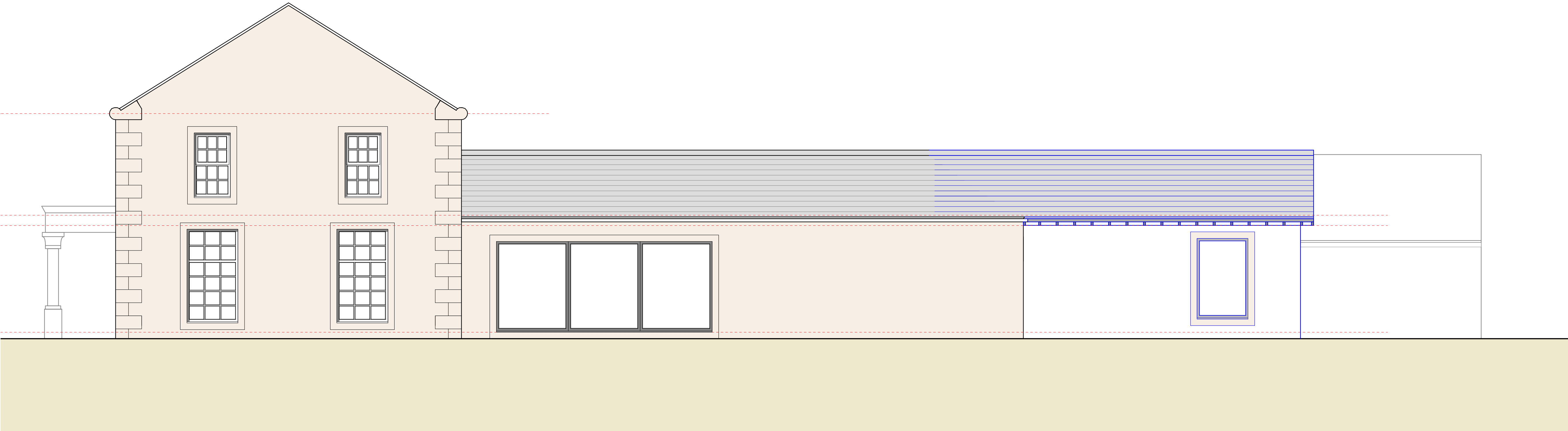
3 ELEVATION - PROPOSED SIDE A (SOUTH FACING) SCALE 1:50 @ A1
