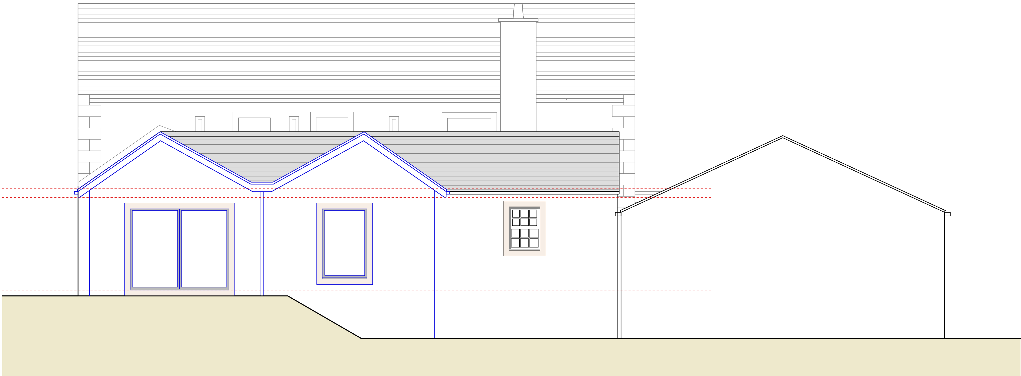
2 ELEVATION - PROPOSED REAR (EAST FACING) SCALE 1:50 @ A1
