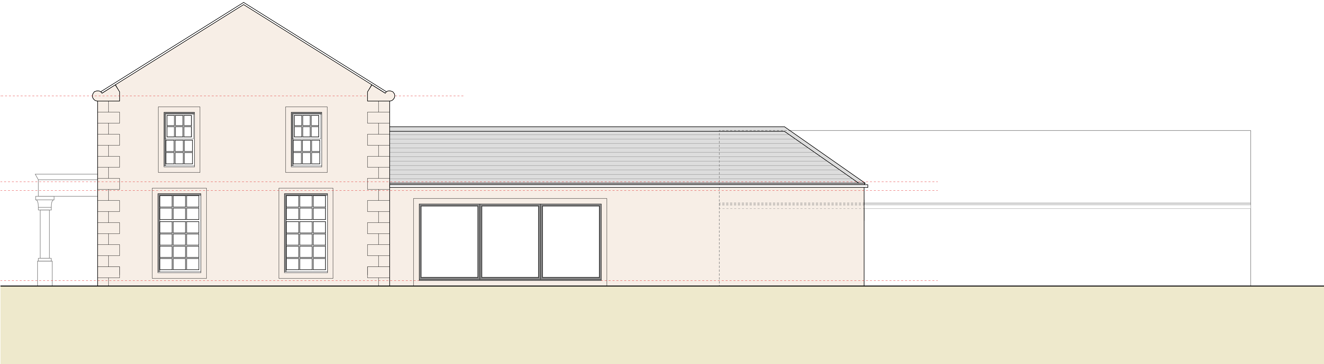
3 ELEVATION - EXISTING SIDE A (SOUTH FACING) SCALE 1:50 @ A1
