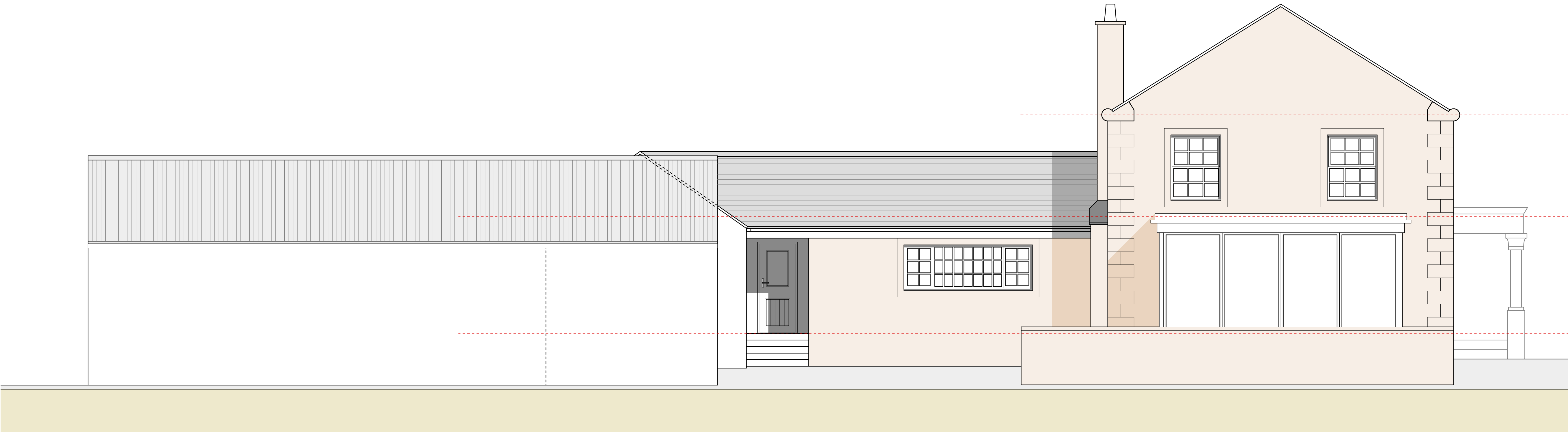
4 ELEVATION - EXISTING SIDE B (NORTH FACING) SCALE 1:50 @ A1
