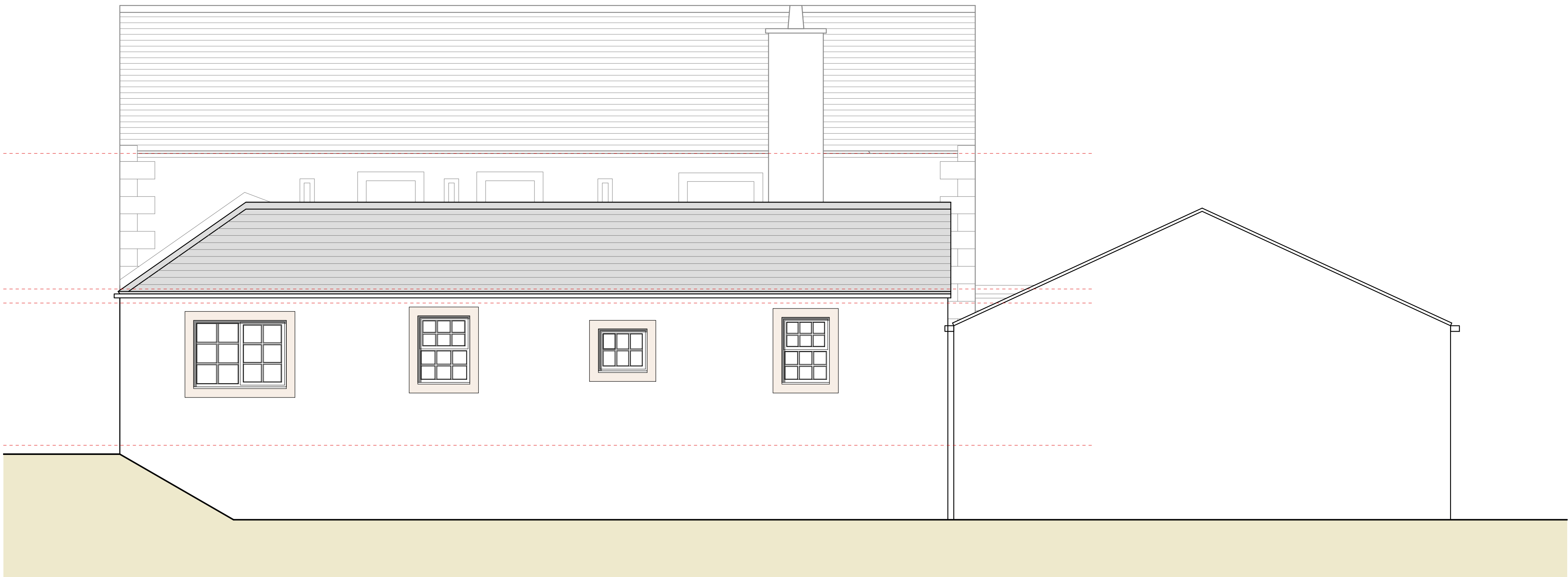
2 ELEVATION - EXISTING REAR (EAST FACING) SCALE 1:50 @ A1
