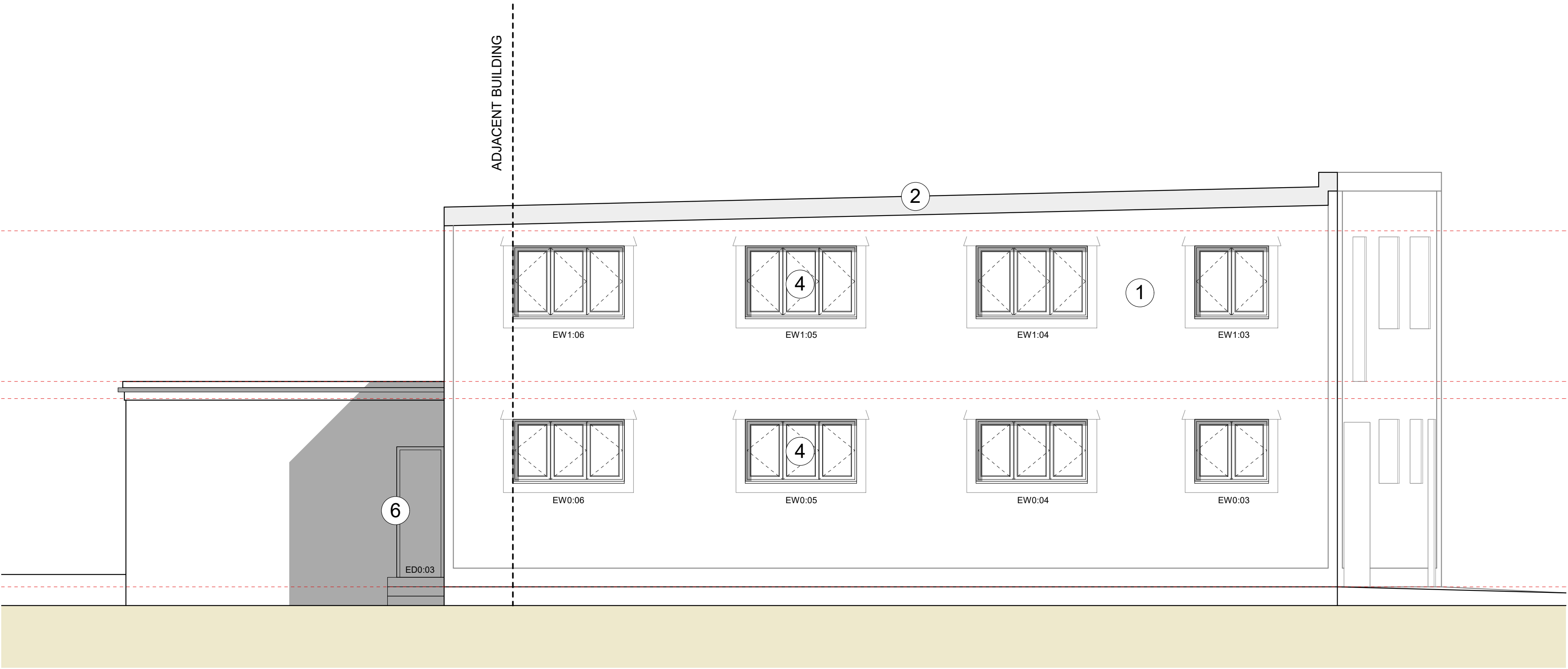
③ ELEVATION - EXISTING SIDE SCALE 1:50 @ A1
