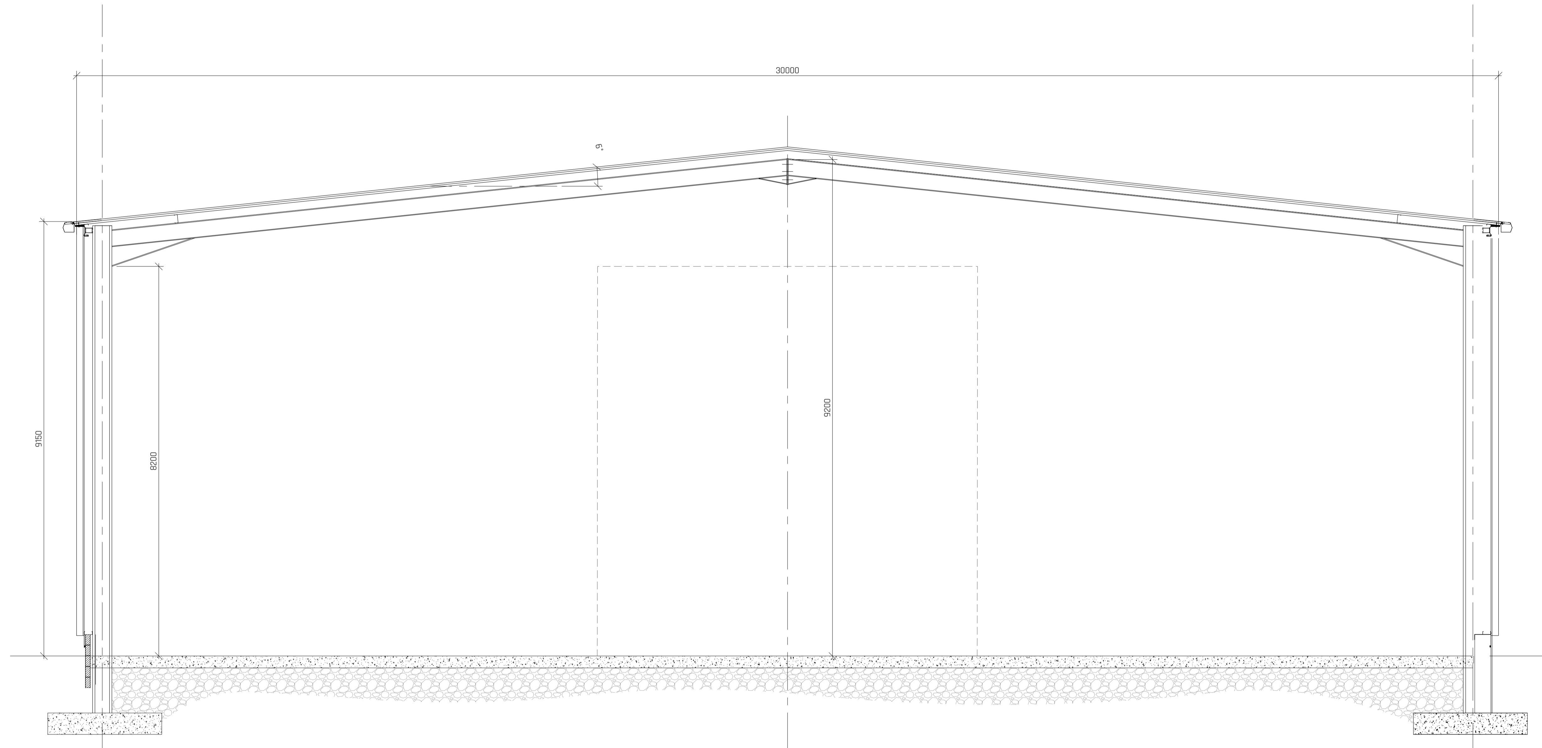
TYPICAL SECTION SCALE 1:50
