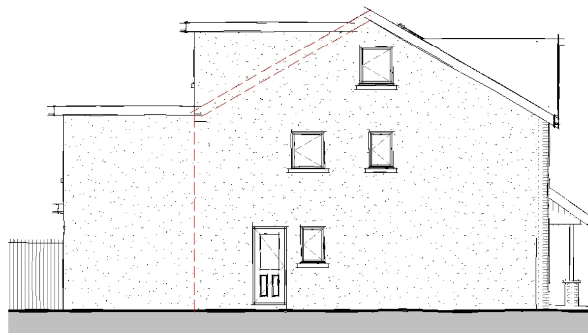
Side Elevation 02
