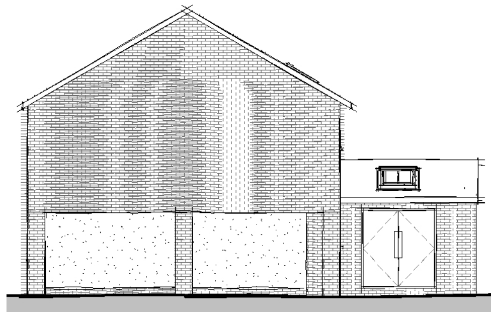
Side Elevation 01
