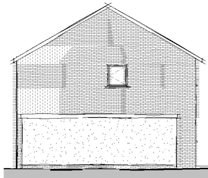
Side Elevation 01
