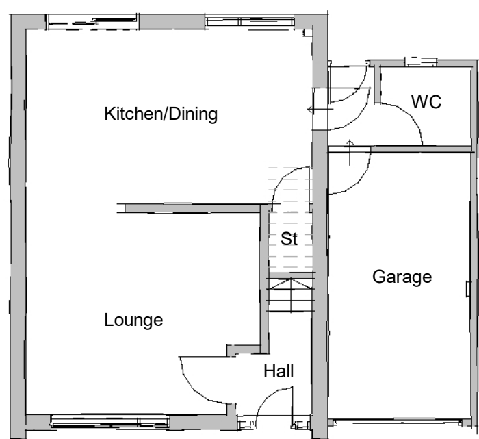
Ground 1 : 100
