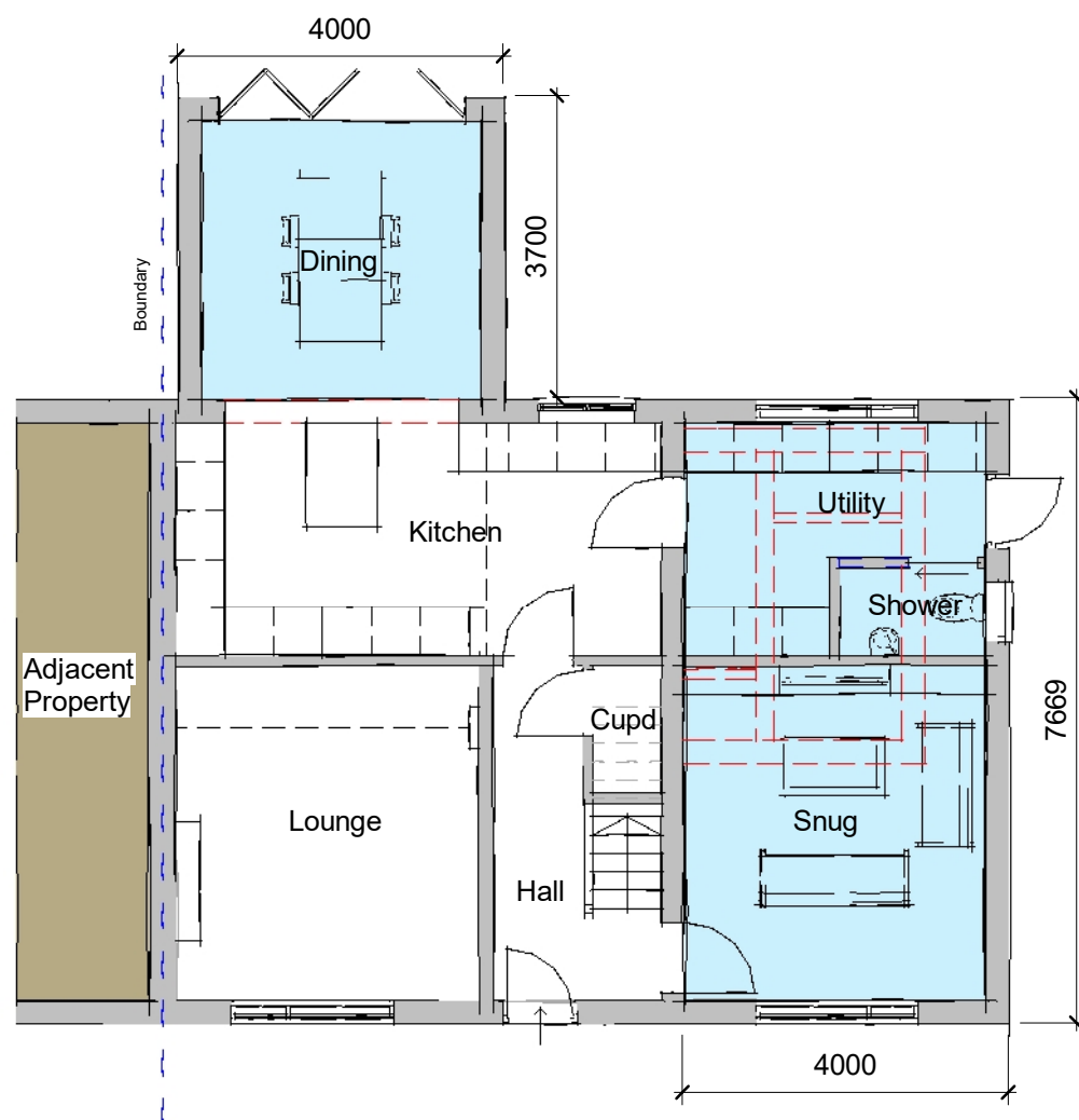
Ground 1 : 100
