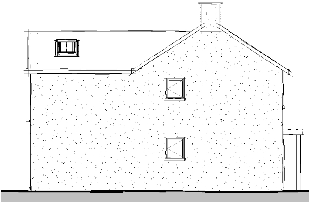
Side Elevation 02 1 : 100
