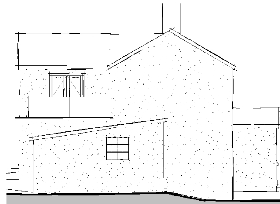
Side Elevation 02
