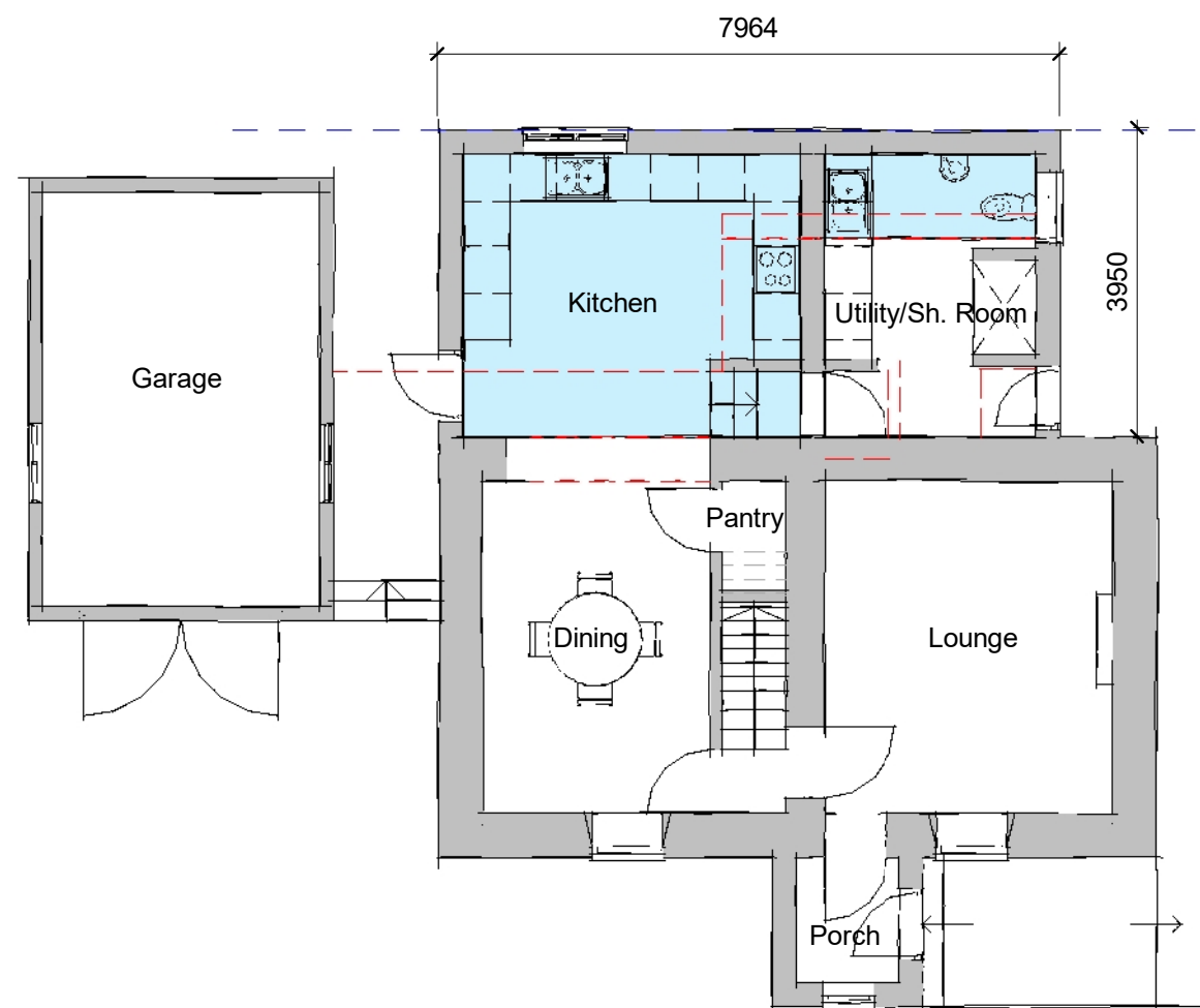
Ground 1 : 100
