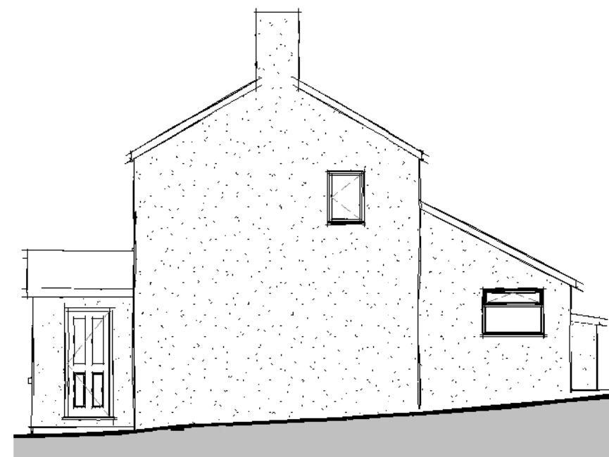
Side Elevation 01
