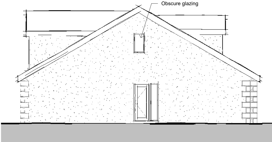
Side Elevation 02 1 : 100
