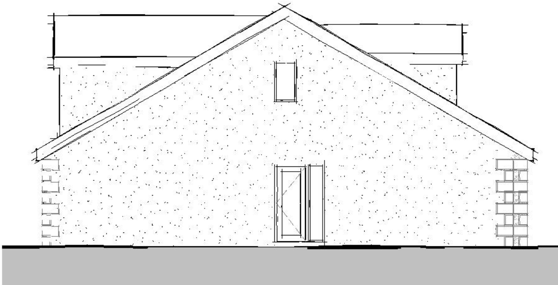
Side Elevation 02 1 : 100
