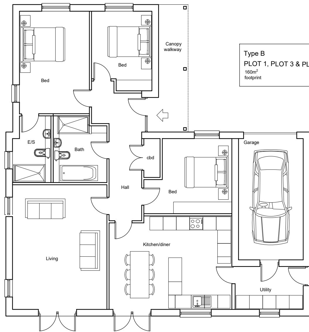
House Plan 1:100
