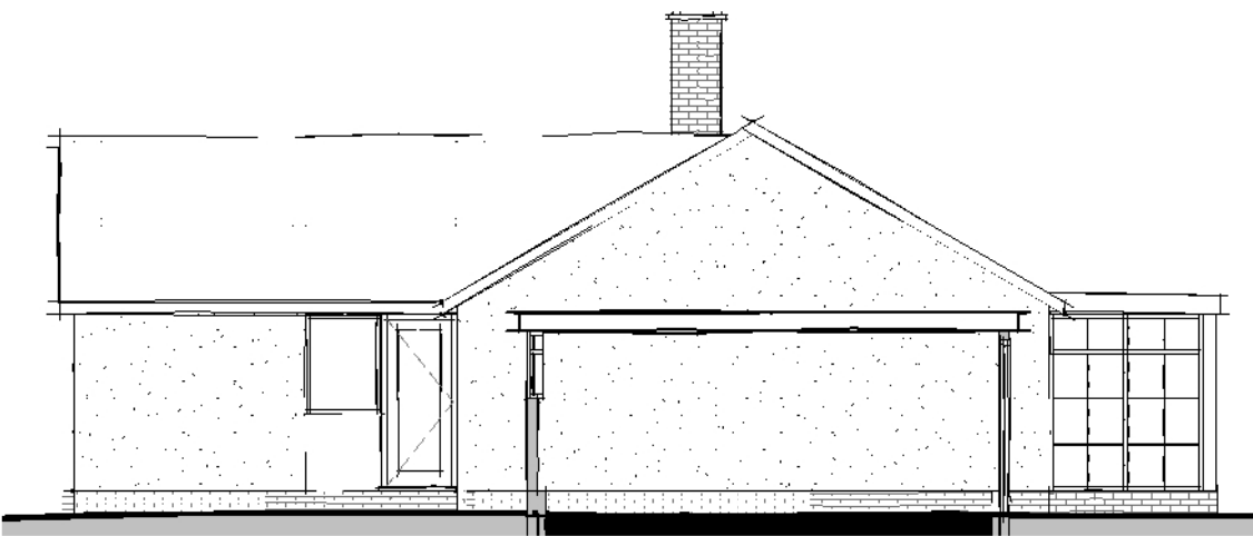
Side Elevation 02
