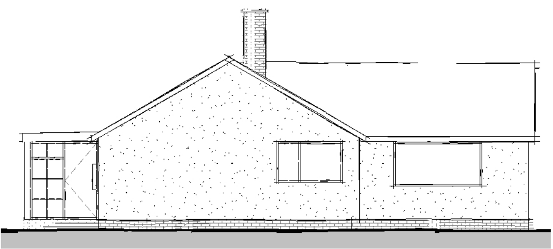
Side Elevation 01
