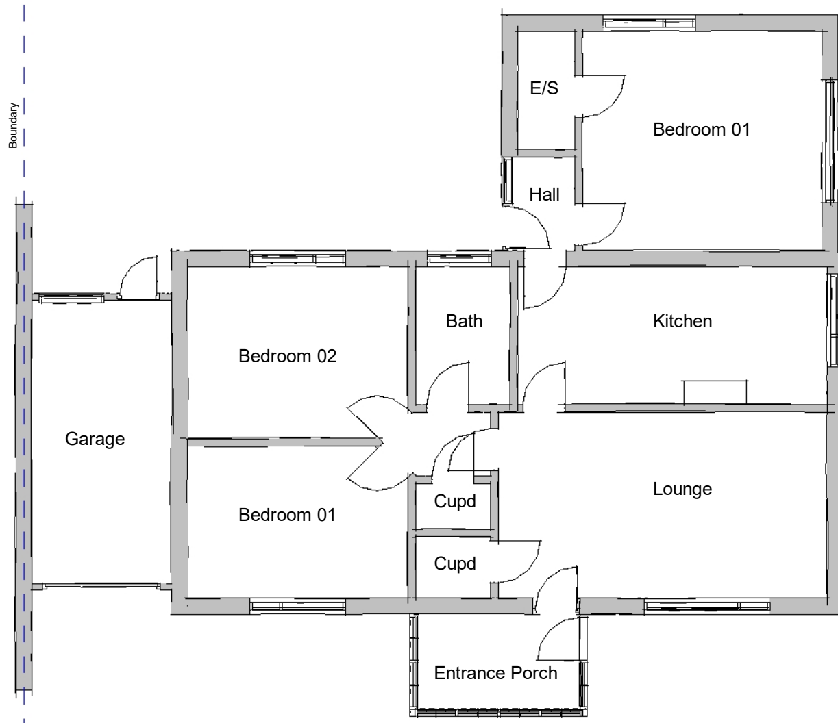
Ground 1 : 100
