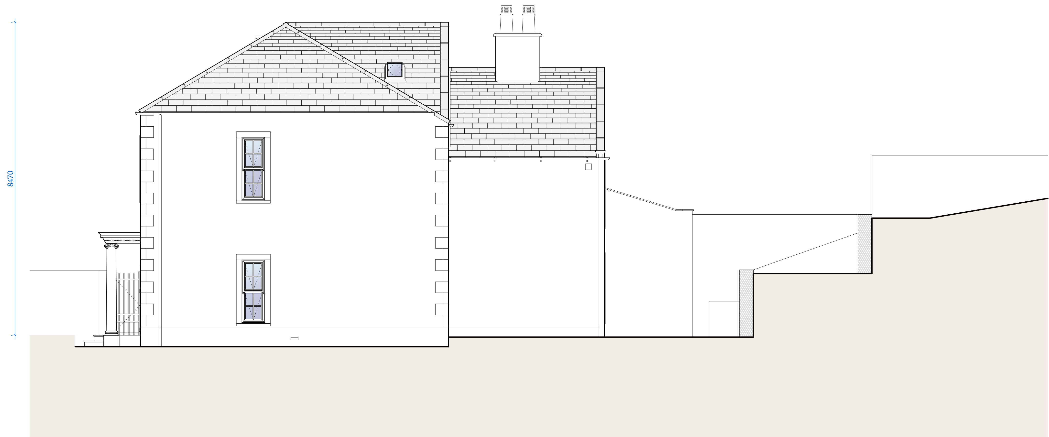
17 Elevation - Side (South-West Facing) Scale - 1 : 50 @ A1
