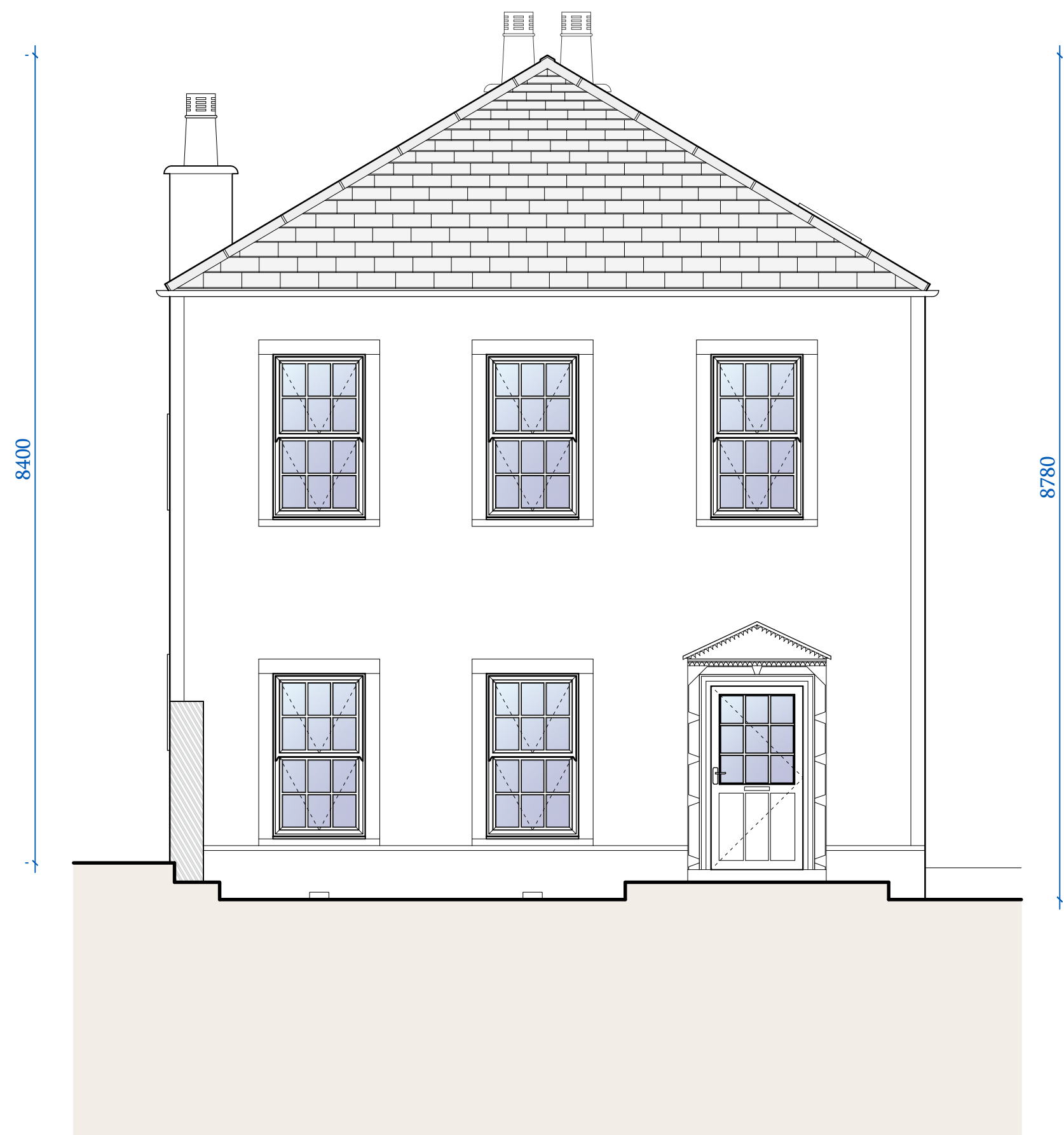
8 Elevation - Front (North-West Facing) Scale - 1 : 50 @ A1
