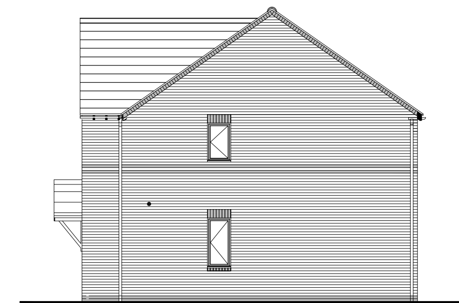
301 SIDE ELEVATION
