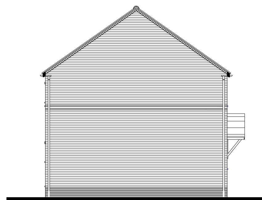
211 SIDE ELEVATION
