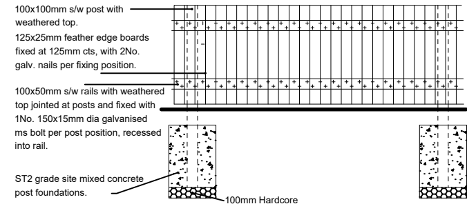
SCREEN FENCE 1.0m max. vertical feather edge boarded fence.
