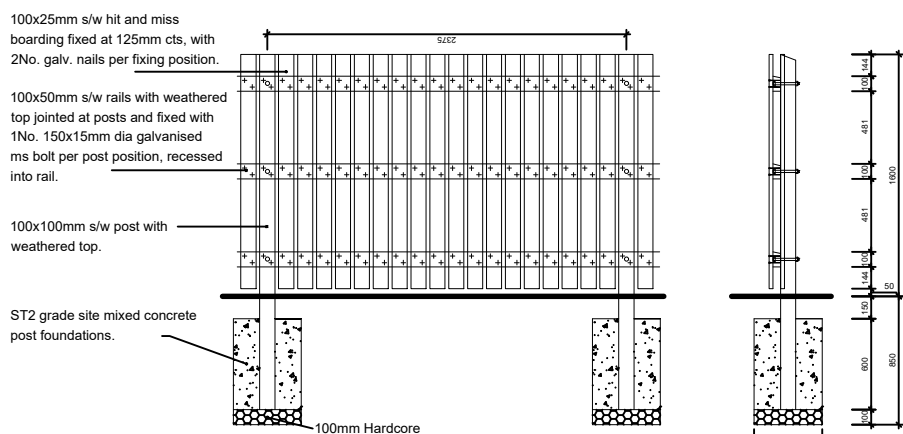
SCREEN FENCE 1.6m Vertical Close Hit and Miss Boarded Fence.
