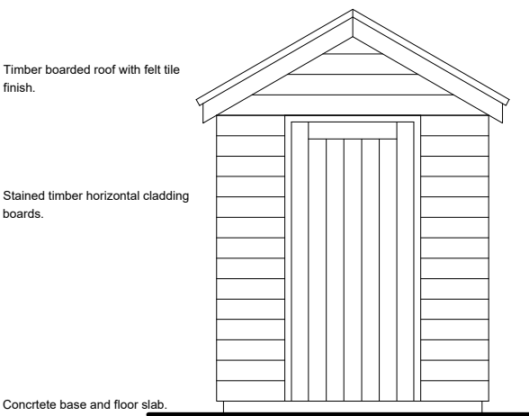
End elevation. GARDEN AND BIKE STORAGE SHED
