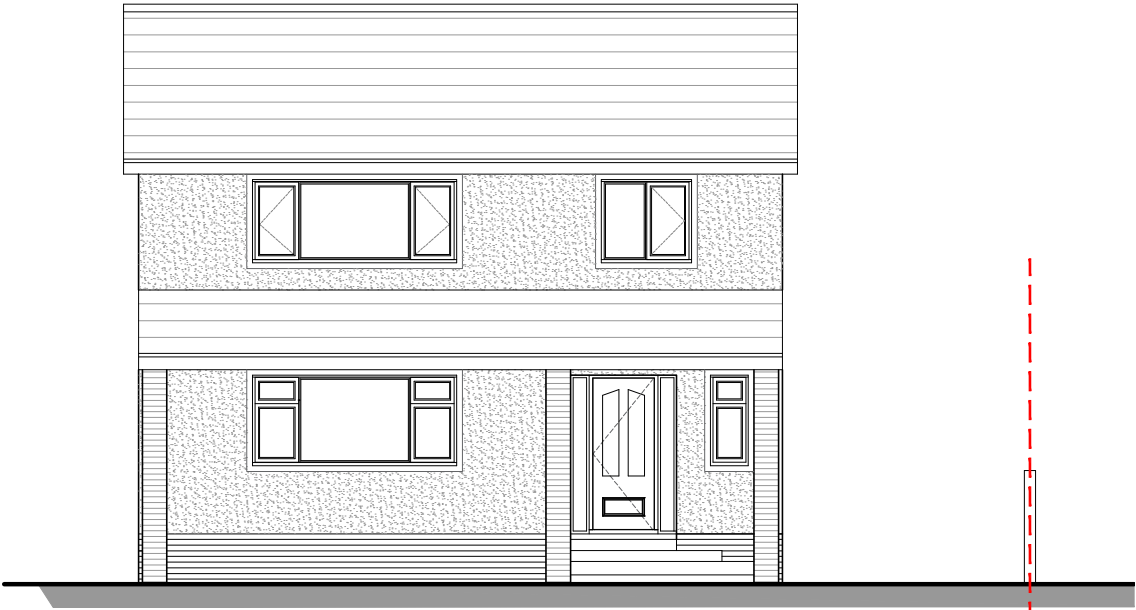
FRONT ELEVATION
