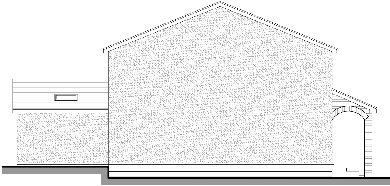
SIDE ELEVATION 02
