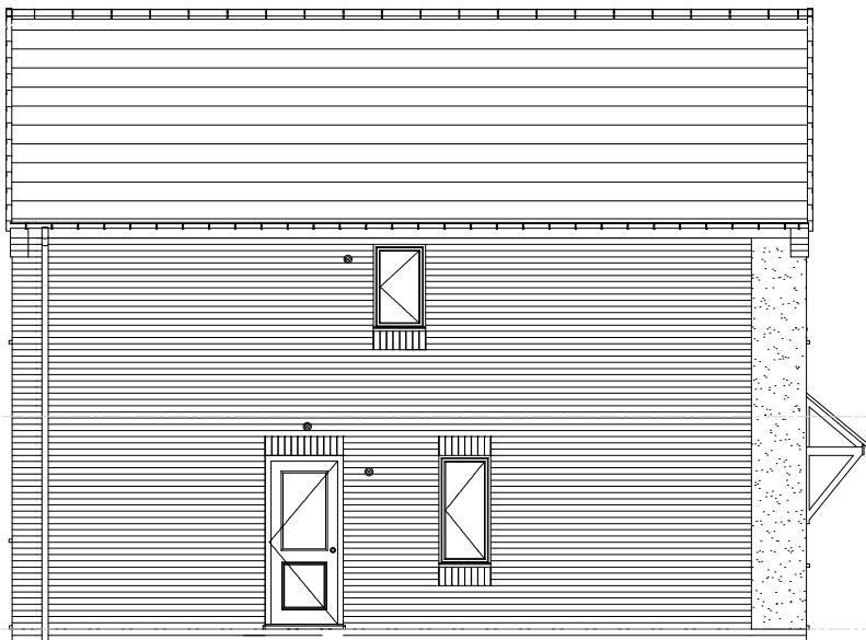
SIDE ELEVATION
