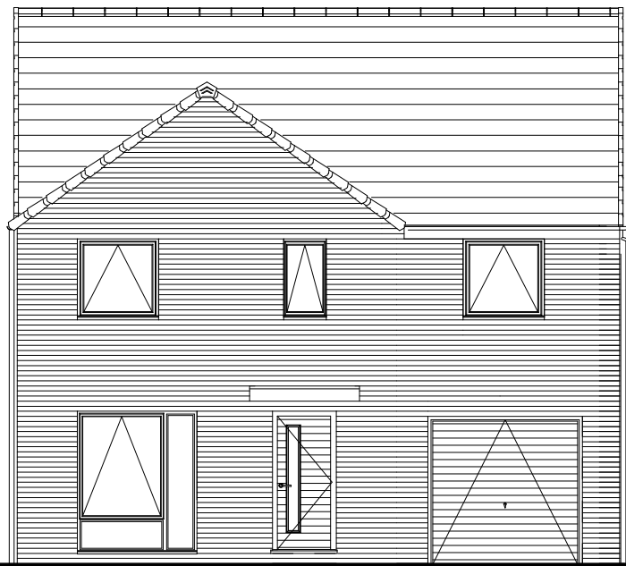
FRONT ELEVATION
