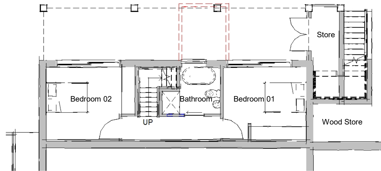
Lower Ground 1 : 100
