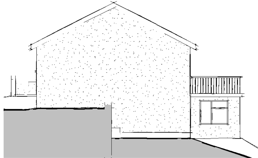
Side Elevation 01
