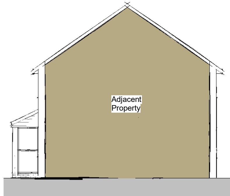
Side Elevation 01
