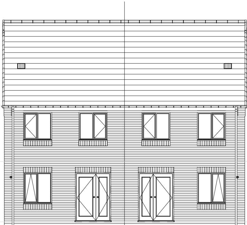
REAR ELEVATION
