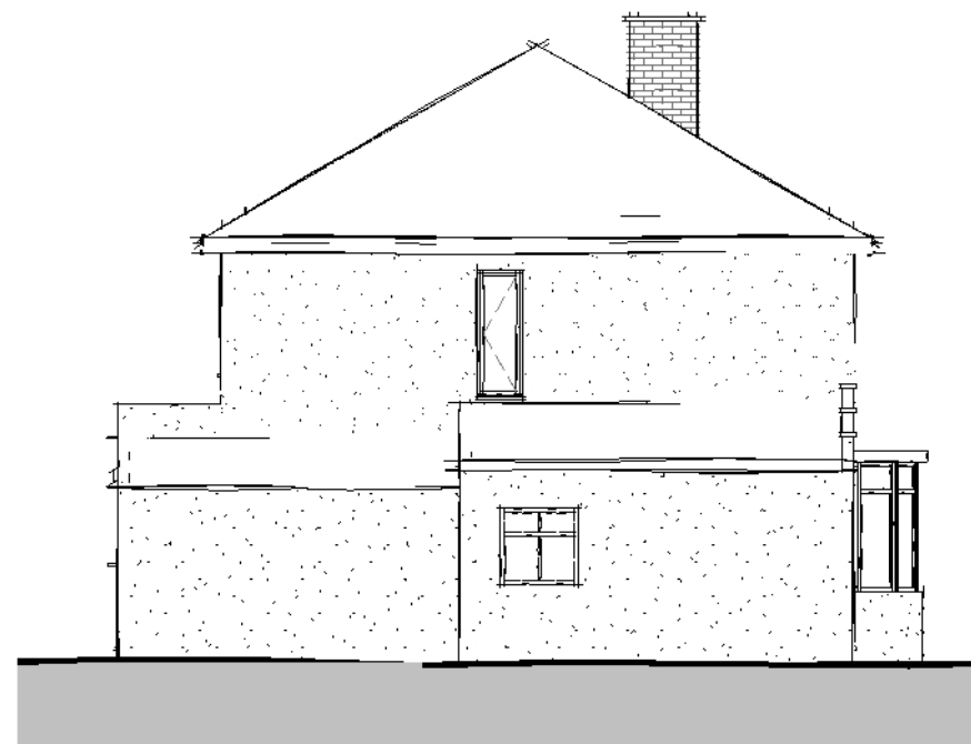
Side Elevation 02
